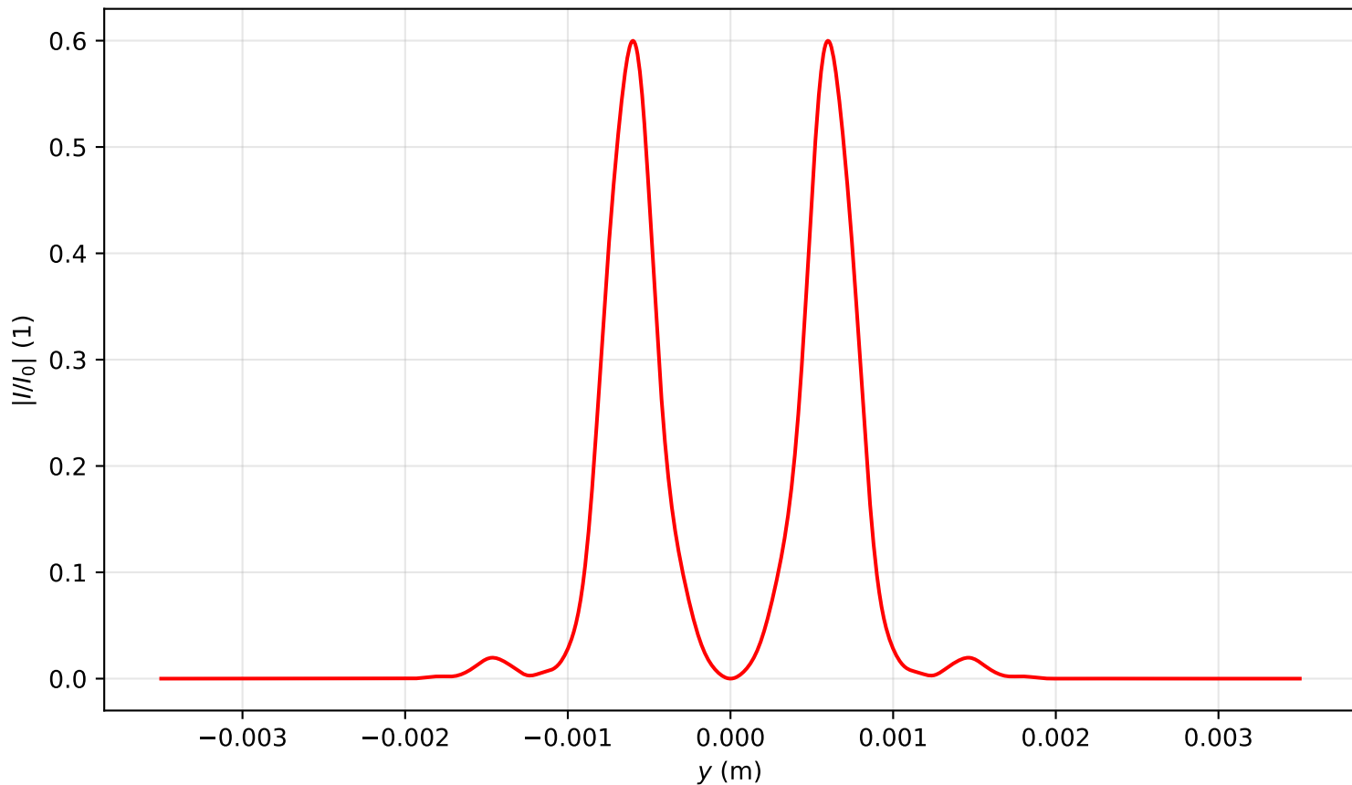
Intensity profile I(x=0, y, z=1.194)/I_0 , P_{in}=6.0P_{cr} , artificial time
